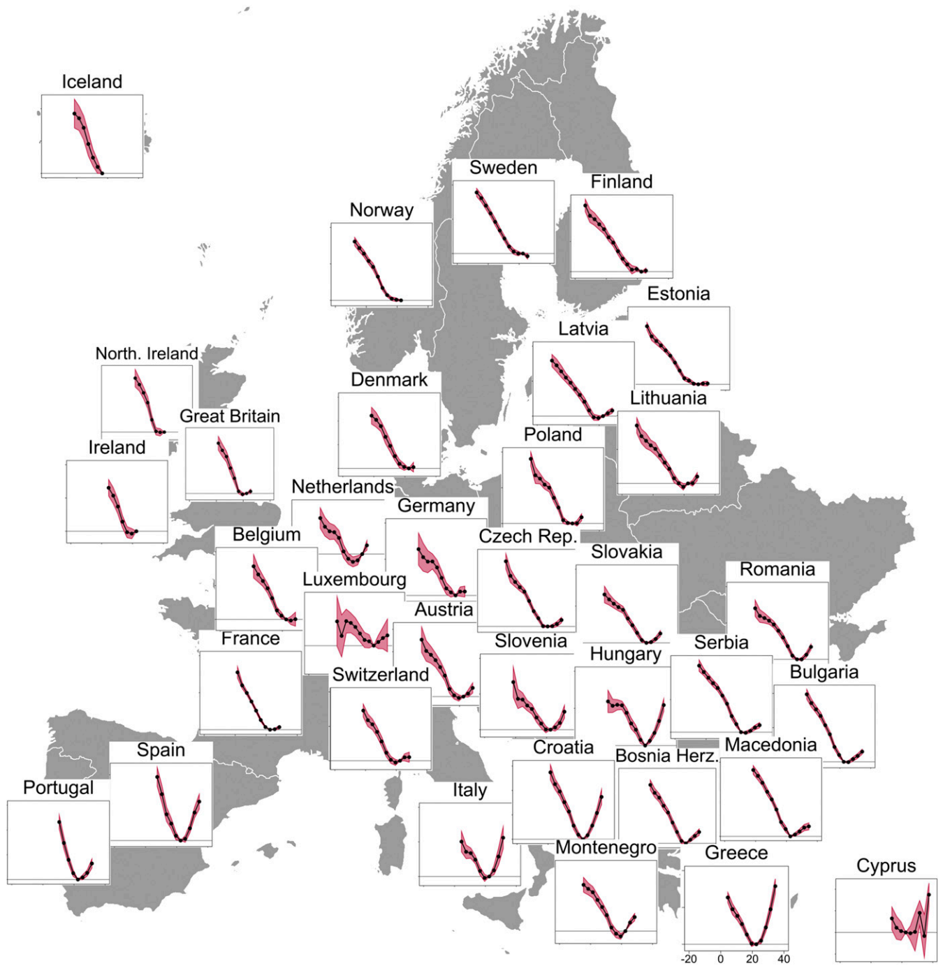
Fig. 1. Similar temperature responses of daily peak load across countries. Response of daily peak load ( y axes, in gigawatts; see SI Appendix, Fig. S1 , for a comprehensive overview of each country's axes scaling) to daily maximum temperature ( x axes, between -20\text{ }^{\circ}\text{C} and +40\text{ }^{\circ}\text{C} ) based on observational data for the years 2006–2012. Black dots represent the effect of replacing a day of daily maximum temperature in the omitted category ( 21\text{ }^{\circ}\text{C} – 24\text{ }^{\circ}\text{C} ) with a day of the relevant maximum temperature (see Methods for details). Pink shaded areas denote 95%-confidence band based on Newey–West standard error. Regression functions of all countries display similar characteristics with minimal peak load values at \sim 22\text{ }^{\circ}\text{C} ( 71.6\text{ }^{\circ}\text{F} ) that increase monotonically in lower and higher temperatures, where data coverage is sufficient. Refer to SI Appendix, Fig. S1 , for a detailed depiction of all country panels including axes titling and scaling.
