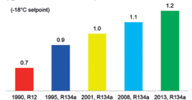
Fig. 3 Coefficient of Performance (COP) improvement for HFC-134a from 1990 to 2013
